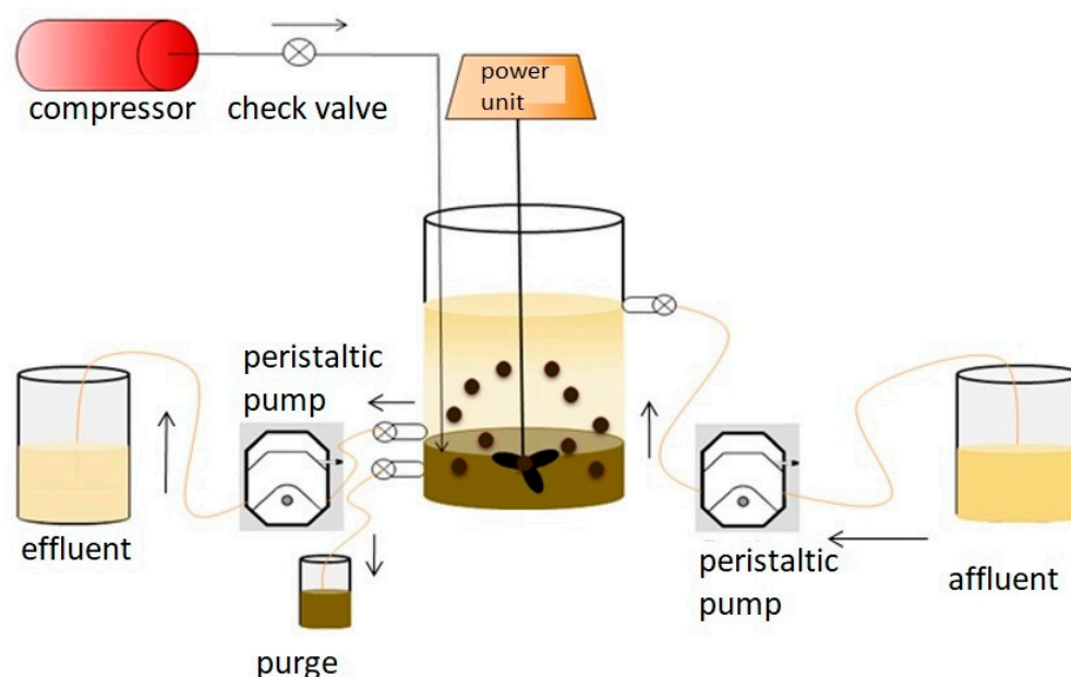
Figure 2. Description of the sequencing batch reactor (SBR).
